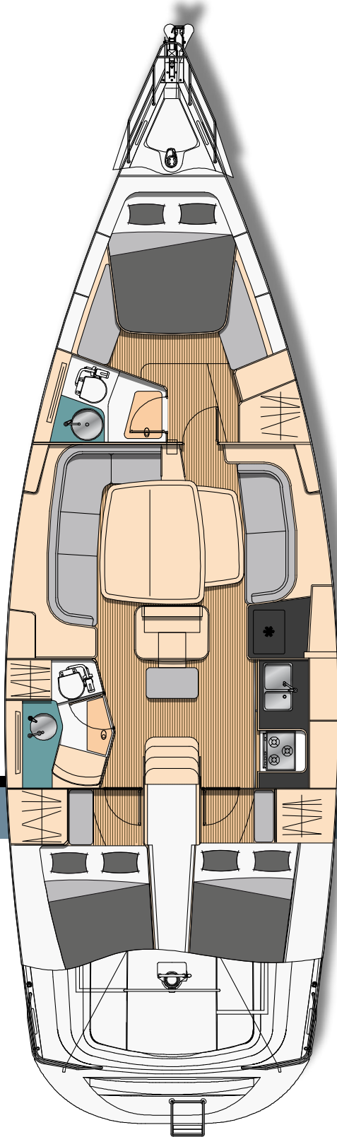
Version 3 cabines - Standard
