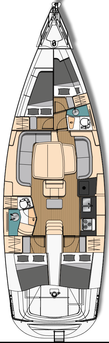
Version 4 cabines - Option
